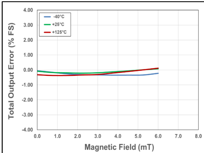
Figure 11. Total Output Error vs. Current vs. Temperature
