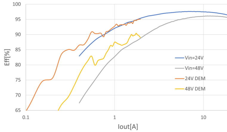
Figure 18. Efficiency typ. @ 240 KHz DEM vs. FPWM
