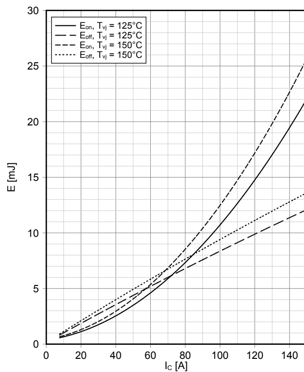
开关损耗 IGBT, 逆变器 (典型) switching losses IGBT, Inverter (typical)
