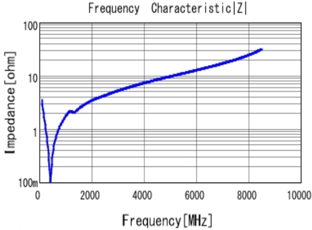
■ GRM1555C1H431GA01 |Z| DC0V, 25degC
