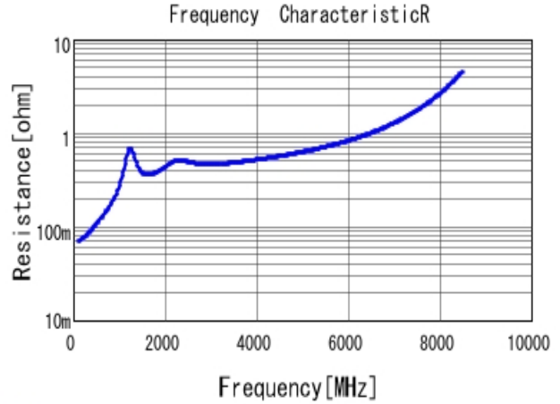
■ GRM1555C1H431GA01 R DC0V, 25degC
