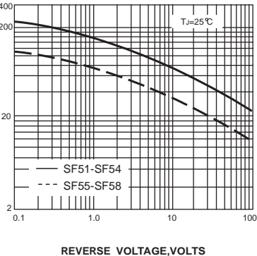
FIG. 5-TYPICAL JUNCTION CAPACITANCE
