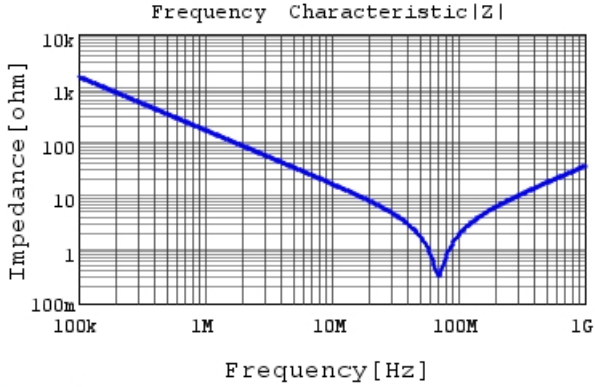
RDER72A102K0P1H03B |Z| DC0V, 25degC
