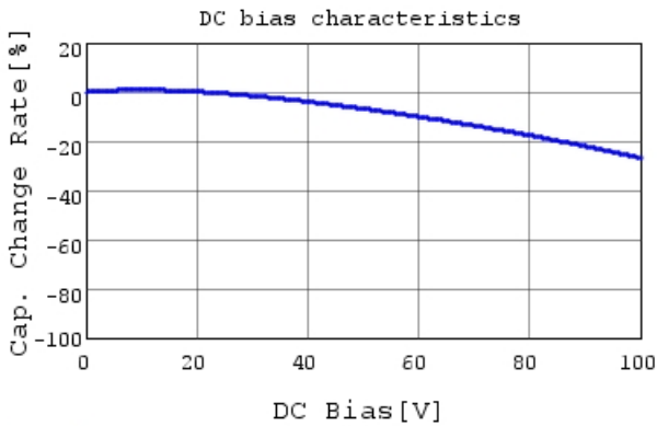
RDER72A102K0P1H03B C-DC bias capchange, 25.0
