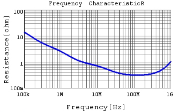
RDER72A102K0P1H03B R DC0V, 25degC
