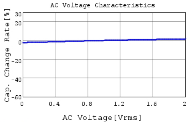
RDER72A102K0P1H03B C-AC Voltage capchange, I
