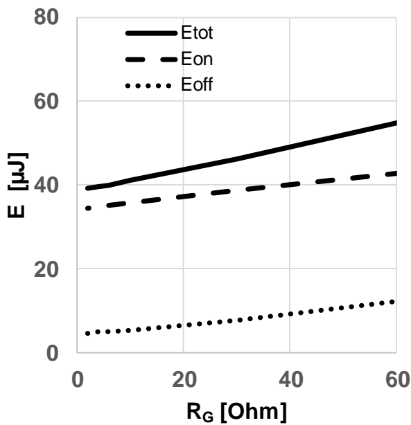
Figure 17 Typical switching energy losses as a function of gate resistance ( E = f(R_{G,ext}), V_{DD} = 800V, V_{GS} = 0V/18V, I_D = 2A, T_{vj} = 175^\circ C, ind. load, test circuit in Fig. E, diode: body diode at V_{GS} = 0V )
