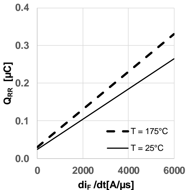
Figure 19 Typical reverse recovery charge as a function of diode current slope ( Q_{rr} = f(di_i/dt), V_{DD} = 800V, V_{GS} = 0V/18V, I_D = 2A, ind. load, test circuit in Fig.E, body diode at V_{GS} = 0V )
