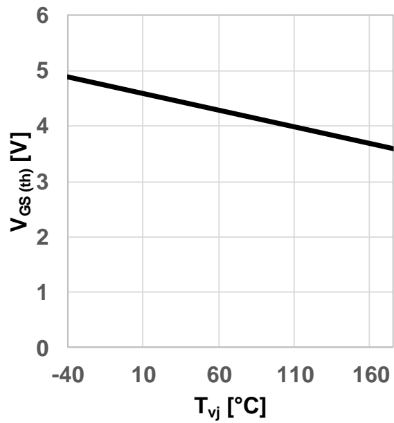
Figure 6 Typical gate-source threshold voltage as a function of junction temperature ( V_{GS(th)} = f(T_{vj}) , I_{DS} = 1\text{mA} , V_{GS} = V_{DS} )
