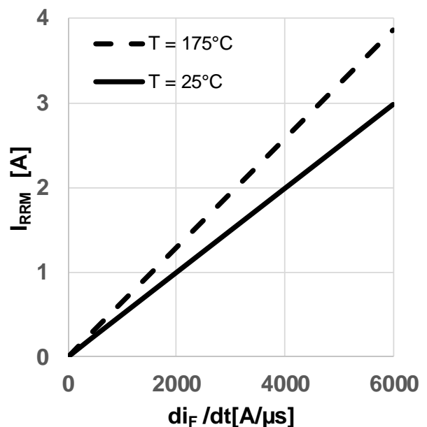
Figure 20 Typical reverse recovery current as a function of diode current slope ( I_{rrm} = f(di_i/dt), V_{DD} = 800V, V_{GS} = 0V/18V, I_D = 2A, ind. load, test circuit in Fig.E, body diode at V_{GS} = 0V )
