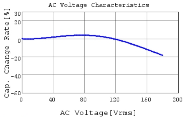
RDER72H105MUB1H03B C-AC Voltage capchange, I
