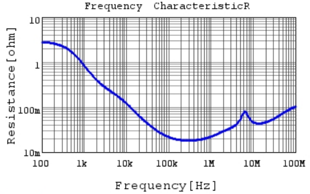
RDER72H105MUB1H03B R DC0V, 25degC
