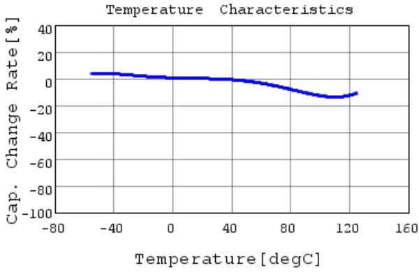
RDER72H105MUB1H03B C-Temp. capchange, DCOV,
