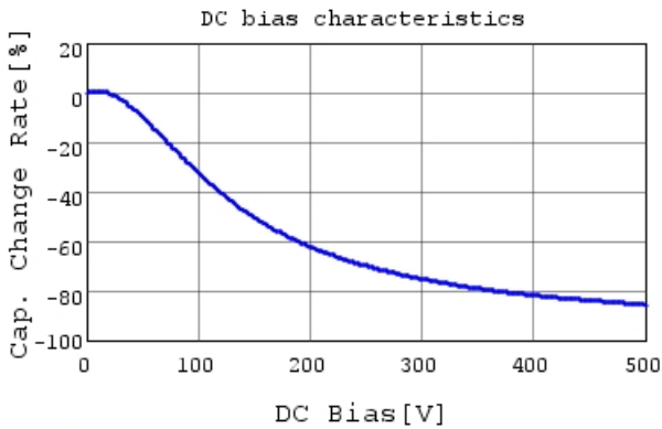
RDER72H105MUB1H03B C-DC bias capchange, 25.0
