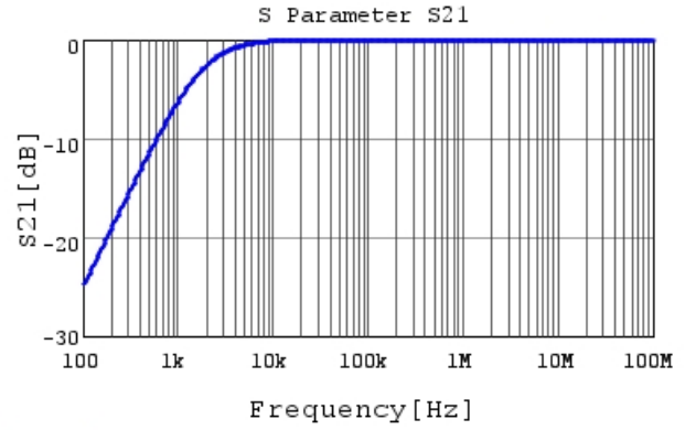
RDER72H105MUB1H03B S21 DCOV, 25degC
