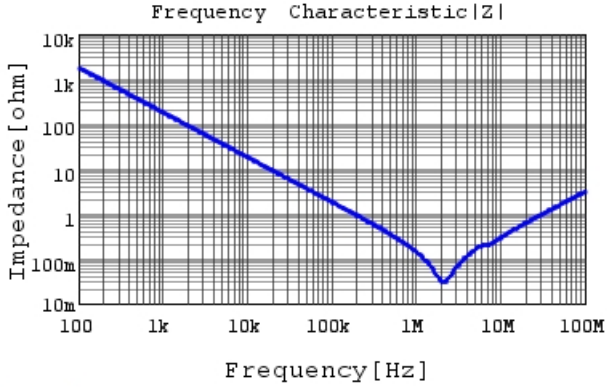
RDER72H105MUB1H03B |Z| DC0V, 25degC
