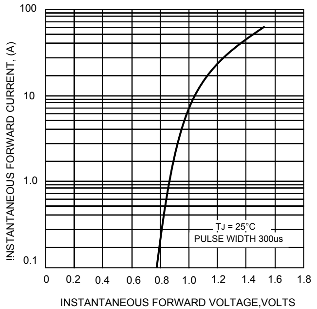
FIG.4-TYPICAL FORWARD CHARACTERISTICS
