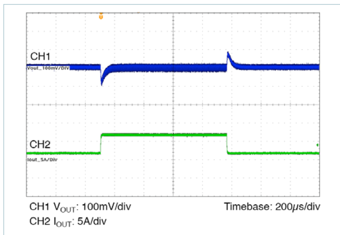
Figure 10 — Transient response 2A to 7A, at 5A/µs
