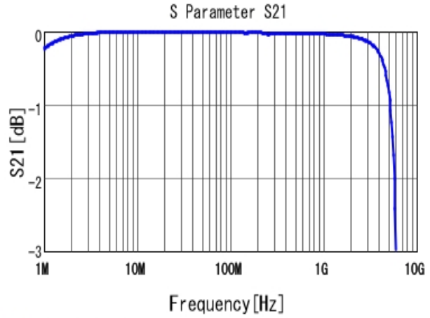
■ GRM3195C1H682JA01 S21 DCOV, 25degC
