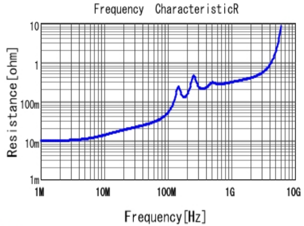
■ GRM3195C1H682JA01 R DCOV, 25degC
