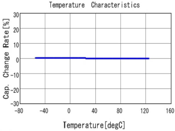
■ GRM3195C1H682JA01 C-Temp. capchange, DCOV, AC1Vrms
