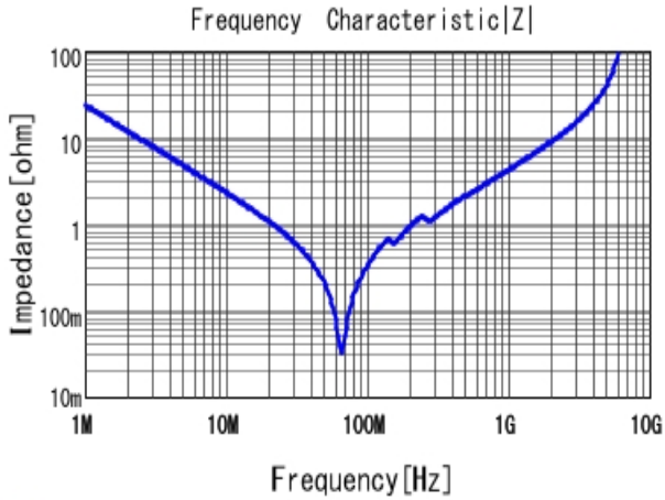
■ GRM3195C1H682JA01 |Z| DCOV, 25degC
