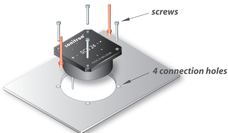
Panel mounting, secured with 4 screws
