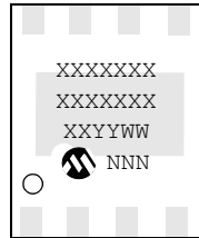
8-Lead DFN (6x5)
