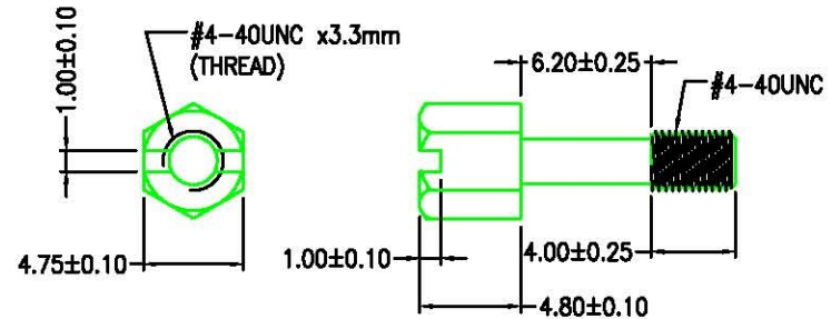
#4-40 UNC Hexscrew SCALE= 2.5:1
