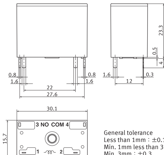
External dimensions
