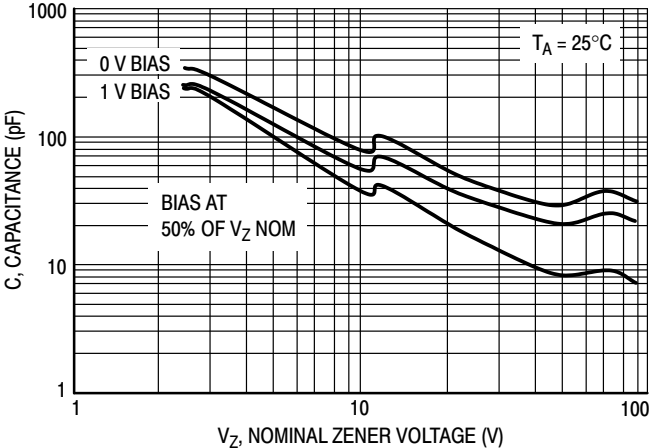
Figure 6. Typical Capacitance
