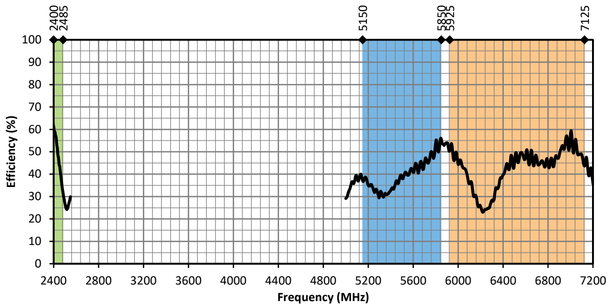
Figure 15. ANT-W63-CW-RCS-ccc Antenna Efficiency, on Edge of Ground Plane
