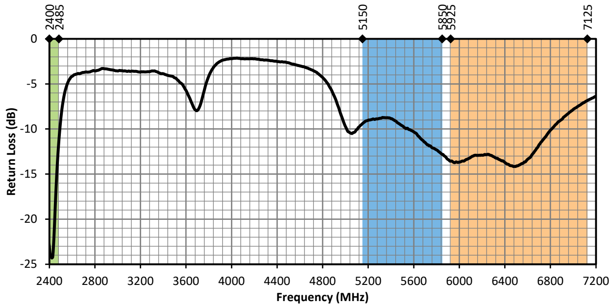
Figure 5. ANT-W63-CW-RCS-ccc Return Loss, Free Space
