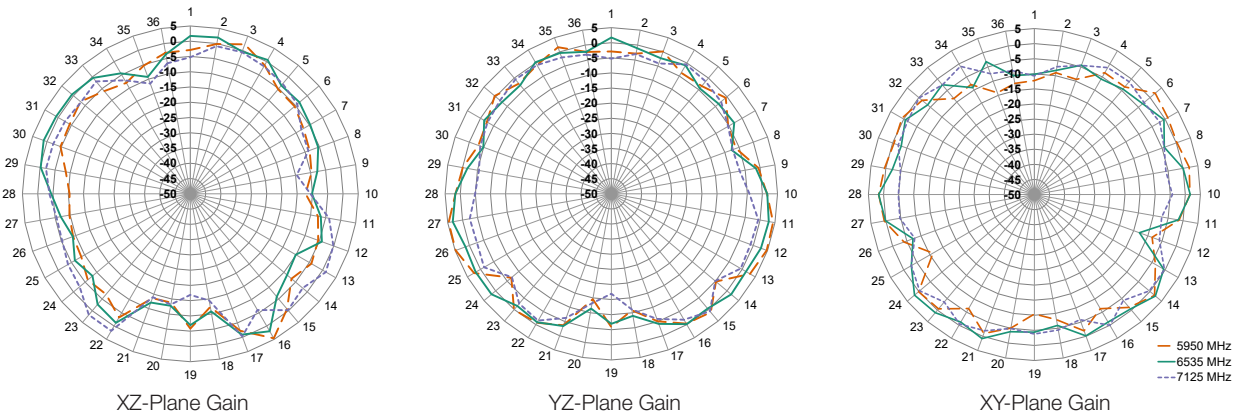
Figure 9. ANT-W63-CW-RCS-ccc Radiation Patterns, Free Space
