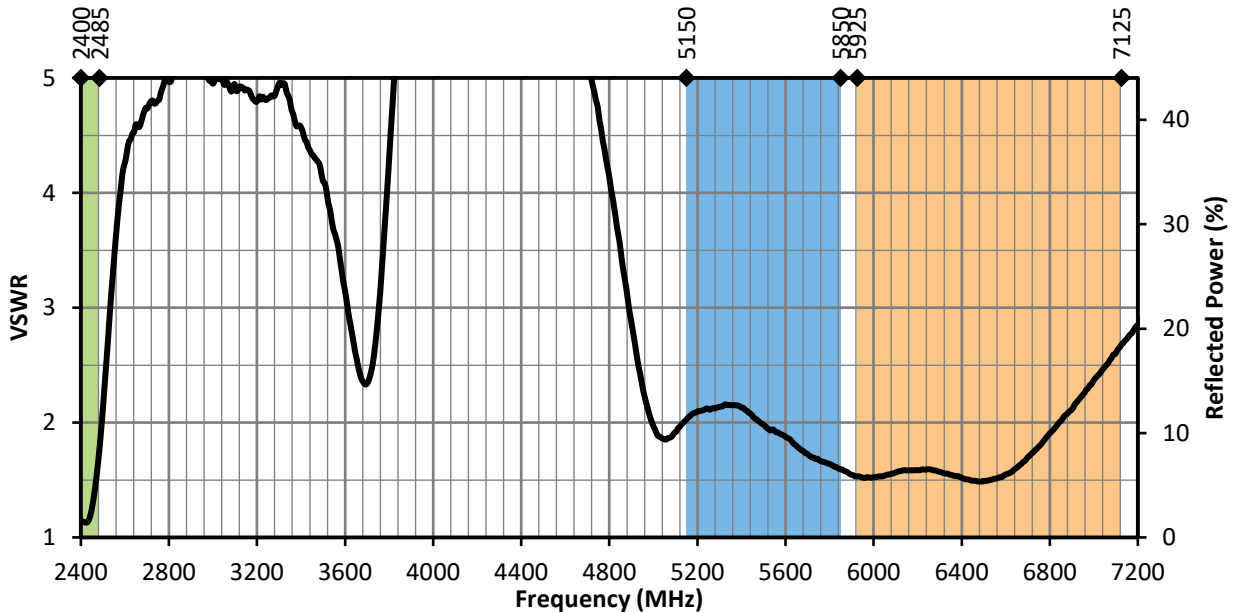
Figure 4. ANT-W63-CW-RCS-ccc Antenna VSWR, Free Space
