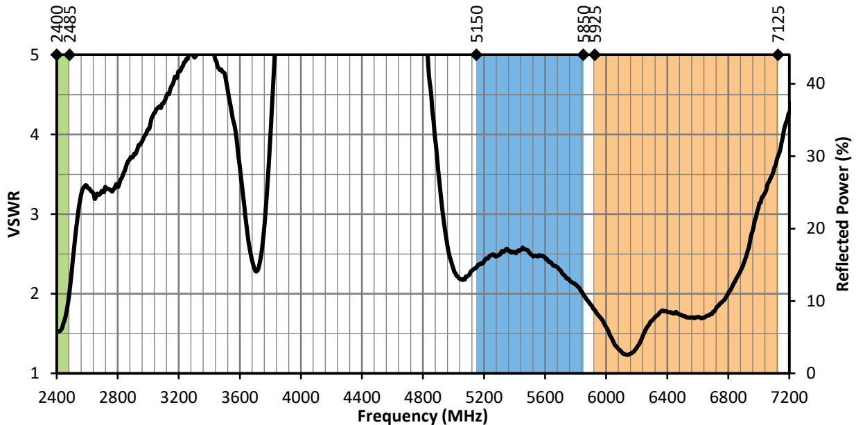
Figure 11. ANT-W63-CW-RCS-ccc VSWR, on Edge of Ground Plane
