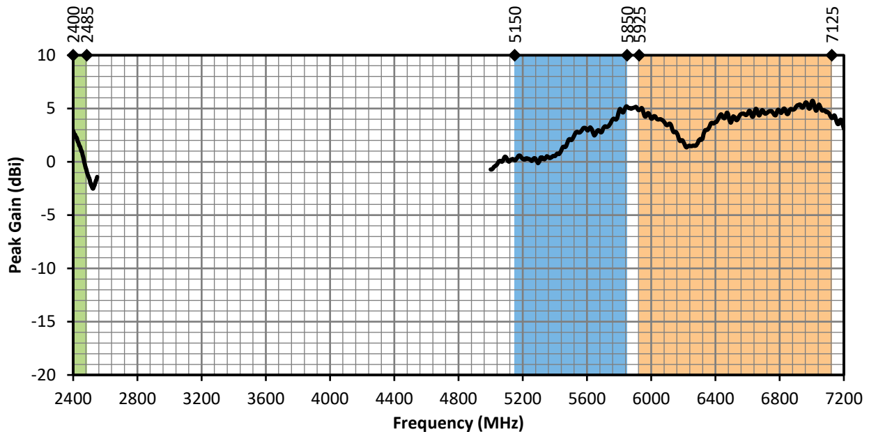
Figure 13. ANT-W63-CW-RCS-ccc Peak Gain, on Edge of Ground Plane
