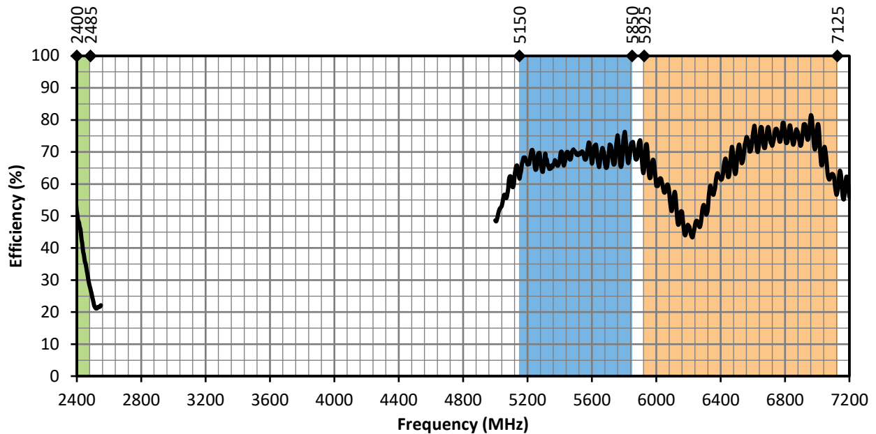
Figure 8. ANT-W63-CW-RCS-ccc Antenna Radiation Efficiency, Free Space
