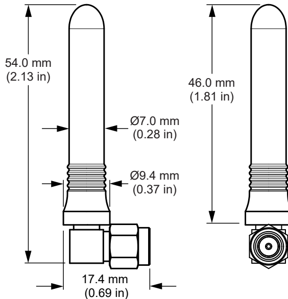
Figure 1. ANT-W63-CW-RCS-ccc Antenna Dimensions
