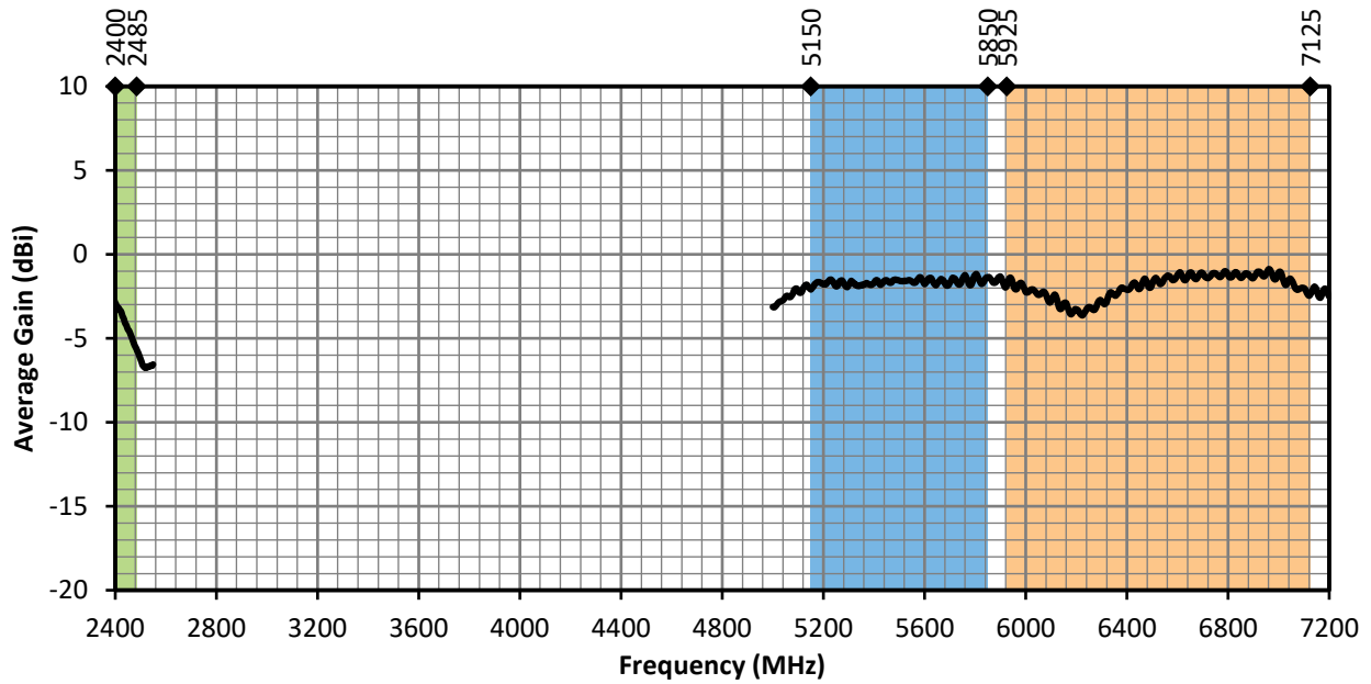
Figure 7. ANT-W63-CW-RCS-ccc Antenna Average Gain, Free Space
