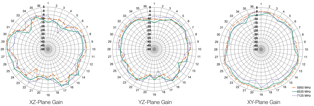
Figure 16. Radiation Patterns for ANT-W63-CW-RCS-ccc, on Edge of Ground Plane
