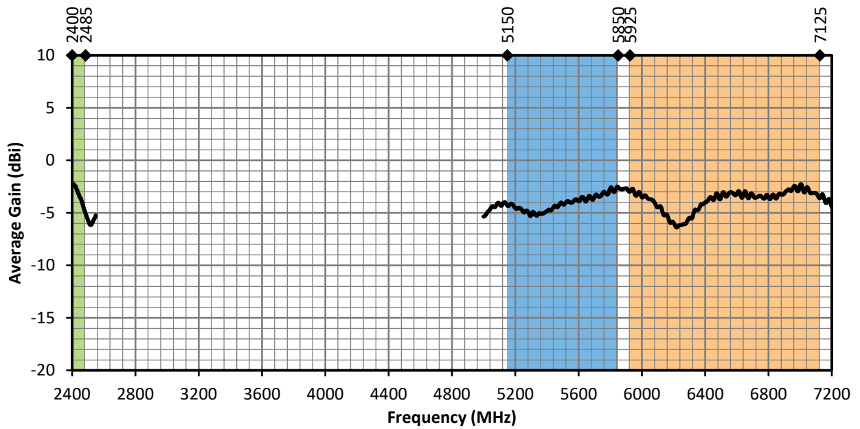
Figure 14. ANT-W63-CW-RCS-ccc Antenna Average Gain, on Edge of Ground Plane
