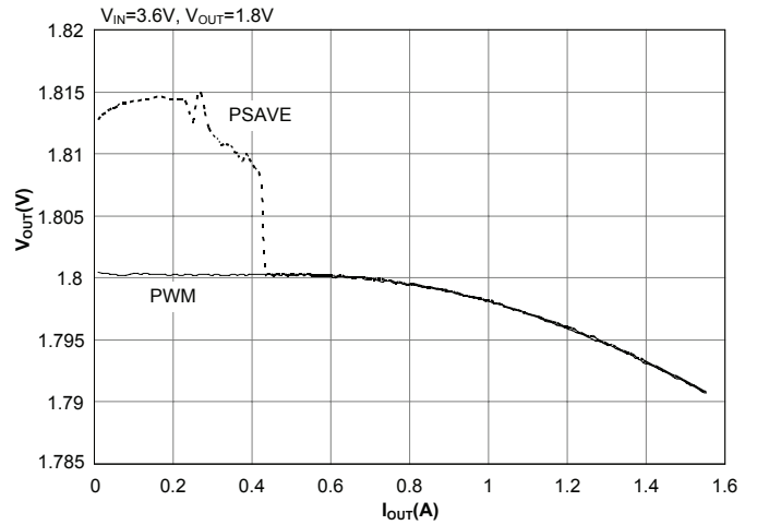
Load Regulation
