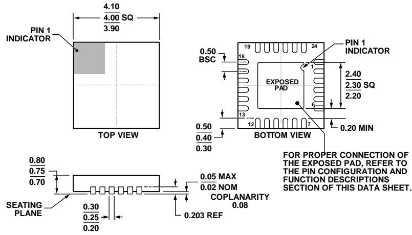
Figure 72. 24-Lead Lead Frame Chip Scale Package [LFCSP] 4 mm x 4 mm Body and 0.75 mm Package Height (CP-24-14) Dimensions shown in millimeters
