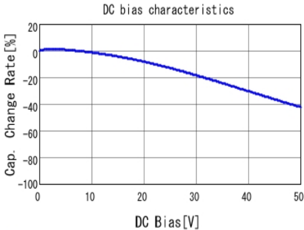
GCM21BR71H104KA37 C-DC bias capchange, 25.0degC, AC1.
