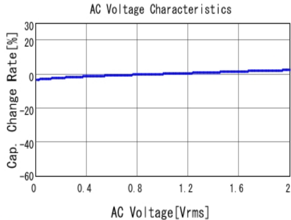
GCM21BR71H104KA37 C-AC Voltage capchange, DCOV, 25.0d
