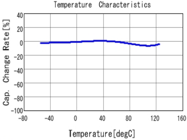
GCM21BR71H104KA37 C-Temp. capchange, DC0.0V, AC1.0V r m
