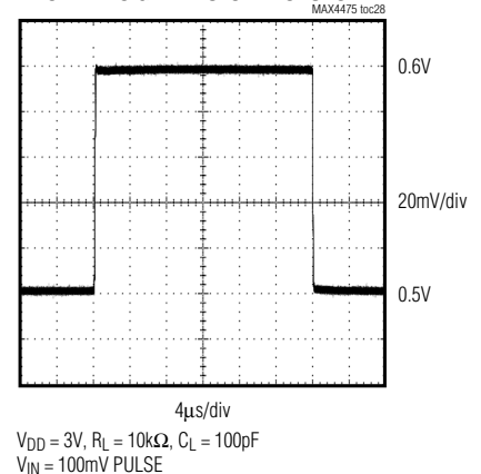
MAX4475-MAX4478 SMALL-SIGNAL PULSE RESPONSE
