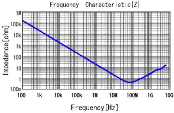
GCJ188R71H103KA01 |Z| DCOV, 25degC
