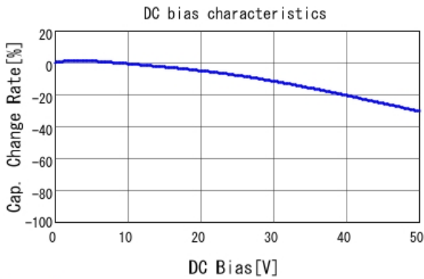
GCJ188R71H103KA01 C-DC bias capchange, 25.0degC, A
