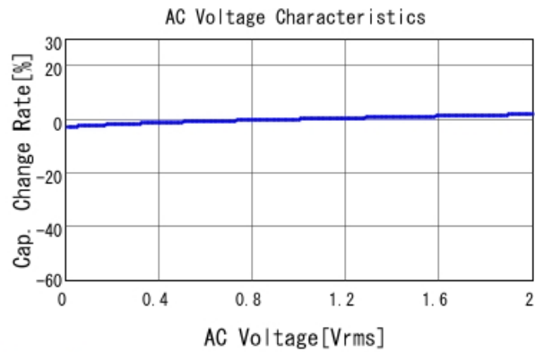
GCJ188R71H103KA01 C-AC Voltage capchange, DCOV, 25
