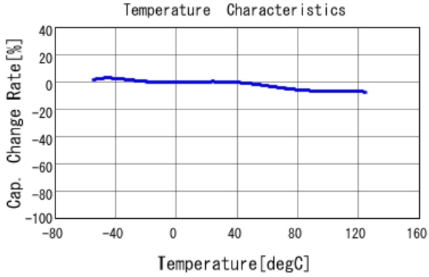
GCJ188R71H103KA01 C-Temp. capchange, DC0.0V, AC1.C
