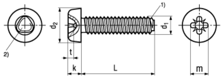
1) Tapered thread end max. 4P 2) Trilobular cross-section
