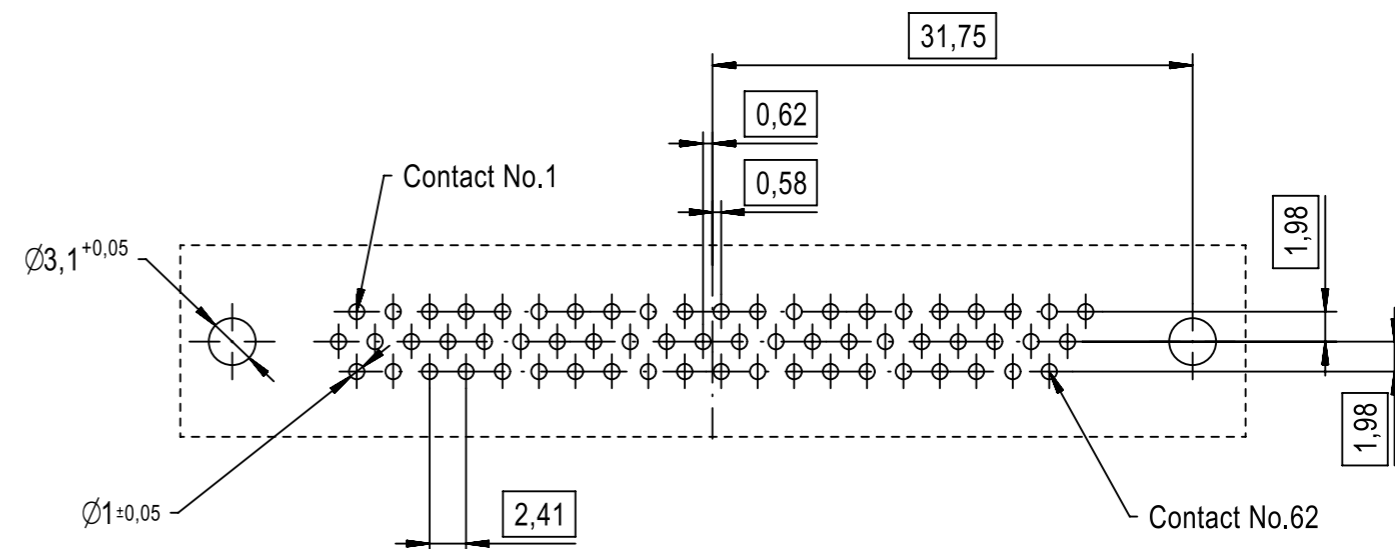
PC-Board layout view component side thickness 1,6 mm
