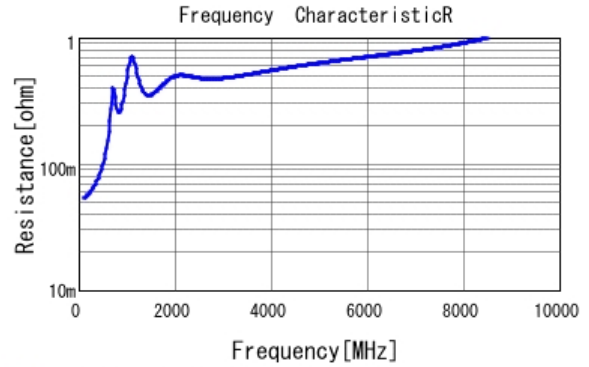
■ GCM1555C1H681JA16 R DCOV, 25degC
