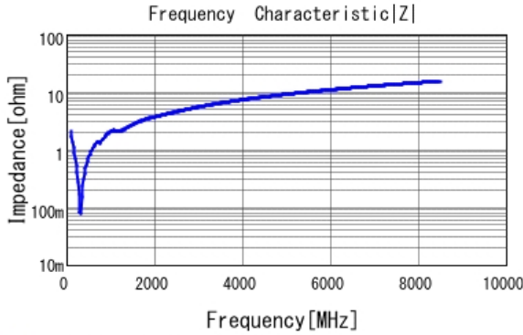
■ GCM1555C1H681JA16 |Z| DCOV, 25degC
