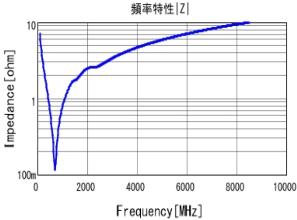
■ GRM0335C1E221JA01 |Z| DC0V, 25degC
