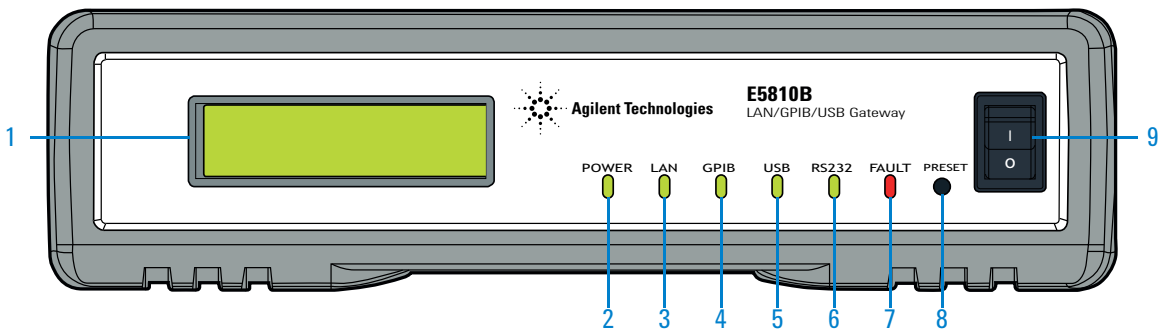
Figure 1-1 E5810B front panel
