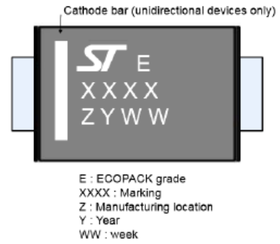
Figure 25. Marking layout
