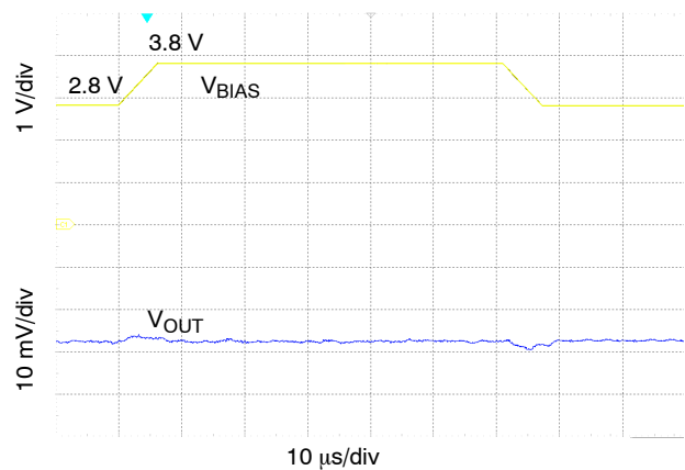
Figure 20. BIAS Line Transient Response, V_{BIAS} = 2.8\text{ V} to 3.8\text{ V} in 5\text{ }\mu\text{s}
