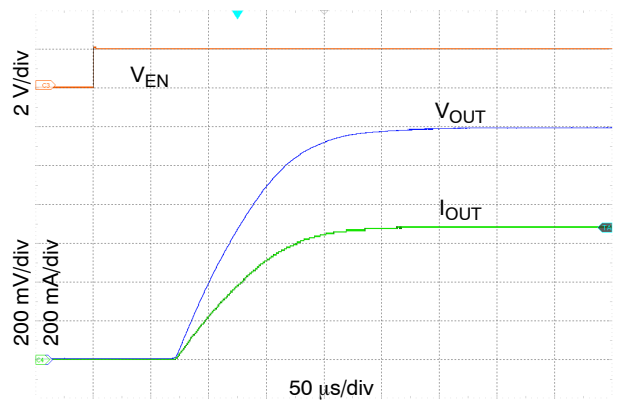
Figure 18. Enable Transient Response, C_{OUT} = 10\text{ }\mu\text{F} , I_{OUT} = 700\text{ mA} – C Option (Slow)
