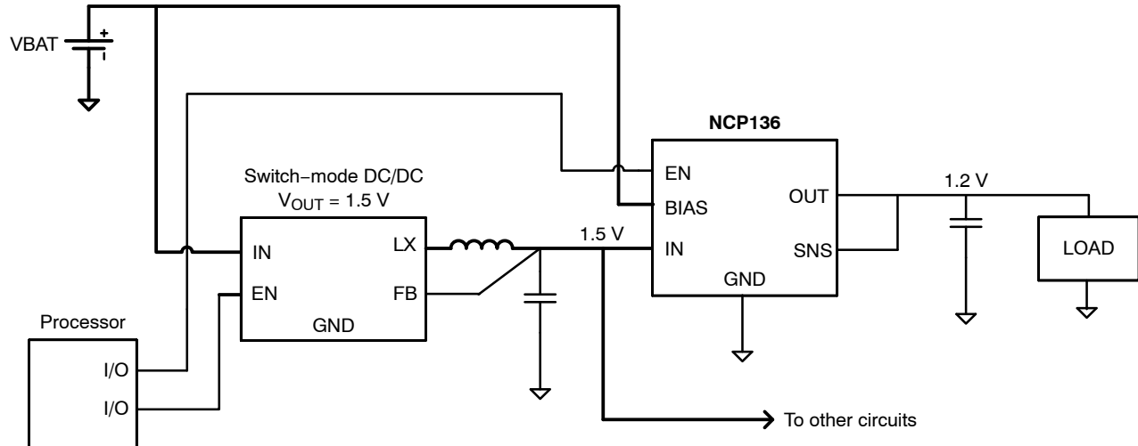
Figure 22. Typical Application: Low-Voltage DC/DC Post-Regulator with ON/OFF Functionality
