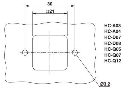
Dimensional drawing
