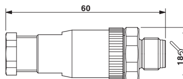
Dimensional drawing
