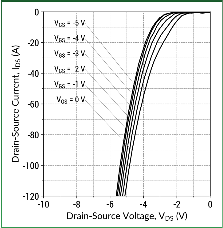
Figure 18: Body Diode Characteristics ( T_j = 175^\circ\text{C} )
