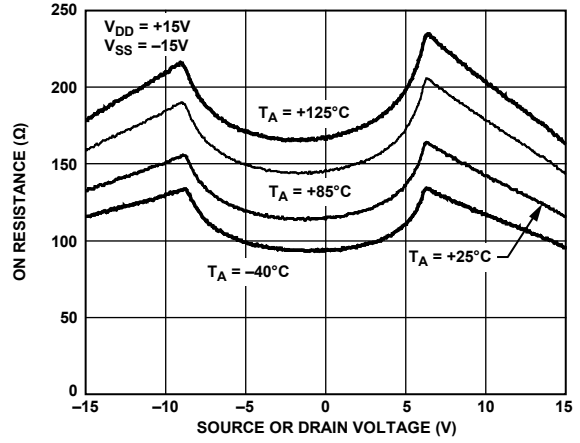
Figure 9. On Resistance vs. Source or Drain Voltage ( V_S or V_D ) for Various Ambient Temperatures ( T_A ), \pm 15 V Dual Supply
