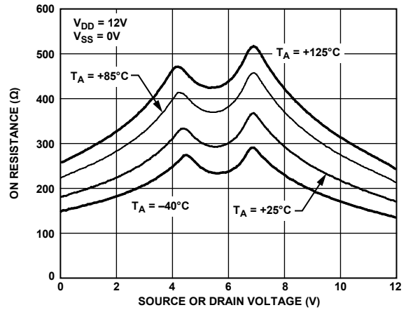
Figure 10. On Resistance vs. Source or Drain Voltage ( V_S or V_D ) for Ambient Temperatures ( T_A ), 12 V Single Supply
