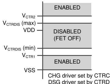
Figure 15. CTRC, CTRD Voltage Levels
