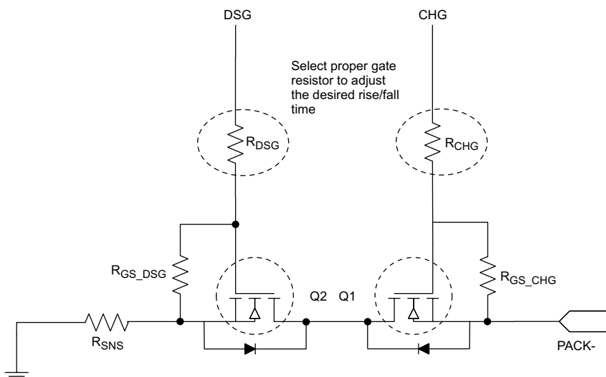
Figure 21. Select Proper Gate Resistor for FET Rise and Fall Time
