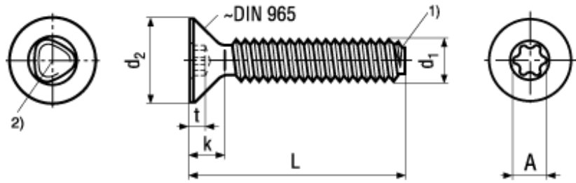
1) Tapered thread end max. 4P 2) Trilobular
