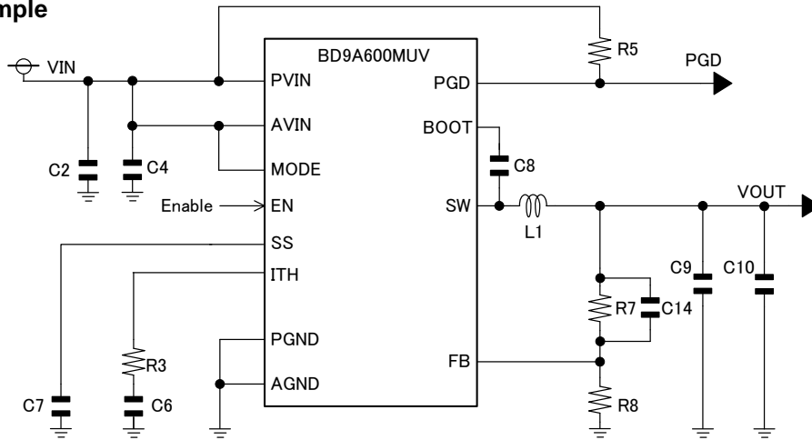
Figure 48. Application Circuit
