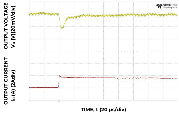
Figure 10. Transient Response to Dynamic Load Change from 50% to 100% at 12Vin, C_{out}=8x47\mu F , C_{Tune}=4.7nF , R_{Tune}=300
