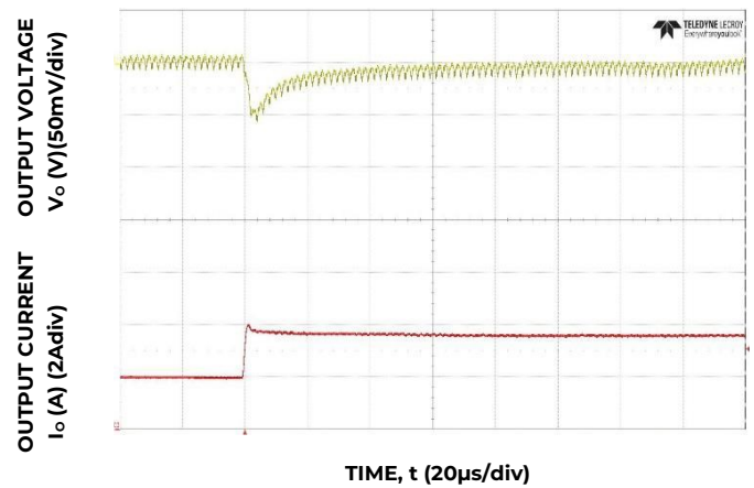
Figure 22. Transient Response to Dynamic Load Change from 50% to 100% at 12Vin, C out =3x47µF, C Tune =1.5nF, R Tune =300
