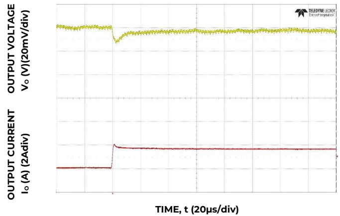
Figure 4. Transient Response to Dynamic Load Change from 50% to 100% at 12V in , C out = 4x47uF + 2x330uF, C Tune =15nF, R Tune =300
