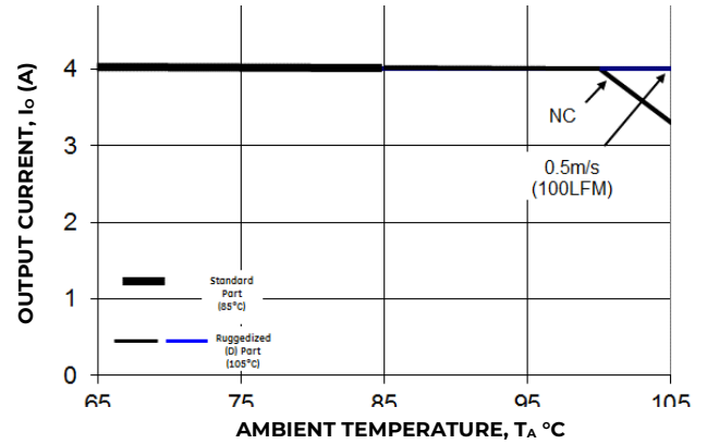
Figure 32. Derating Output Current versus Ambient Temperature
