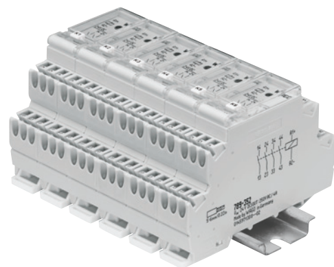
Relay Modules in DIN-Rail Mounted Enclosure 789 Series
