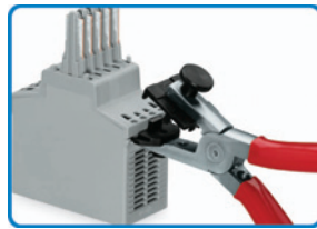
Insert the pliers into the locking slots . . .
