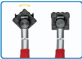
Adjust the pliers to the proper housing width
