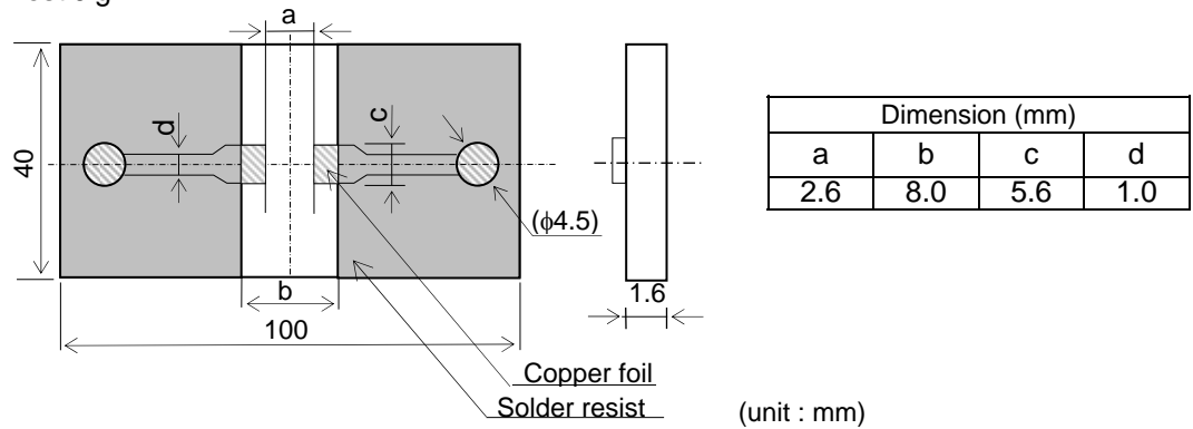
(2) Test Jig B
