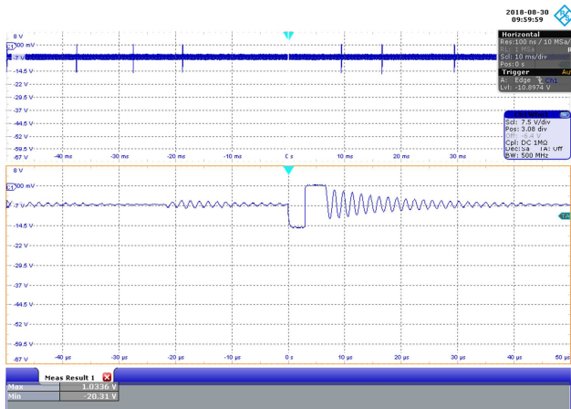
Figure 87 – 85 VAC 60 Hz, No-Load. CH1: 12 V FWL_DIODEF , 7.5 V / div., 10 ms / div. Zoom: 10 μs / div. 12 V PIV MAX = 20.31 V.
