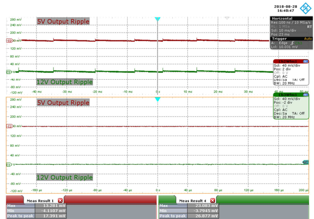
Figure 127 – 115 VAC 60 Hz, 0% Load. CH2: 5 V OUT , 40 mV / div., 10 ms / div. CH3: 12 V OUT , 40 mV / div., 10 ms / div. Zoom: 40 µs / div. 5 V Output Ripple = 17.391 mV. 12 V Output Ripple = 26.877 mV.
