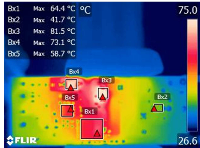
Figure 144 – 230 VAC, Full Load. Bottom Side.
