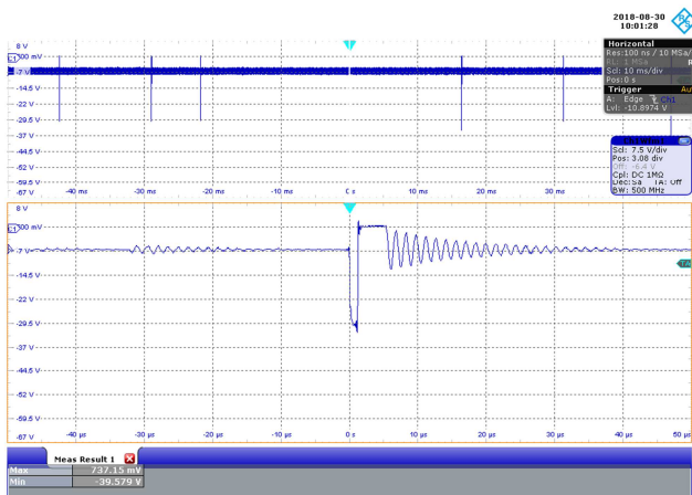
Figure 89 – 230 VAC 50 Hz, No-Load. CH1: 12 V FWL_DIODEF , 7.5 V / div., 10 ms / div. Zoom: 10 μs / div. 12 V PIV MAX = 39.579 V.
