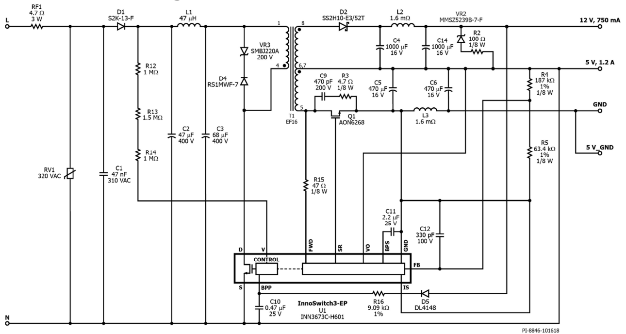
Figure 3 – Schematic Diagram.
