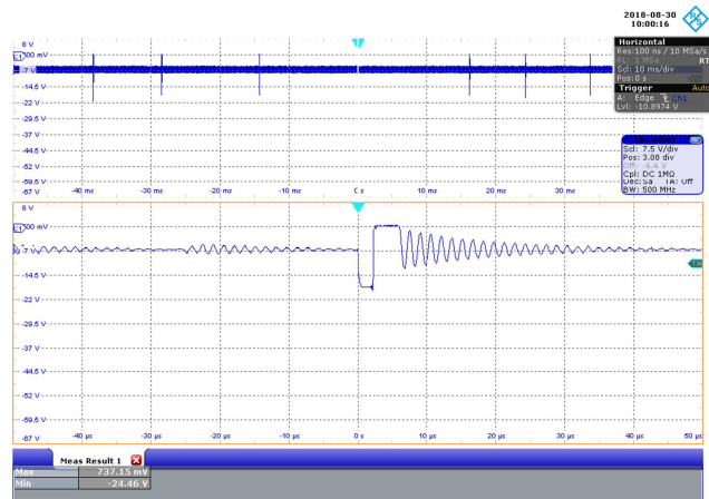
Figure 88 – 115 VAC 60 Hz, No-Load. CH1: 12 V FWL_DIODEF , 7.5 V / div., 10 ms / div. Zoom: 10 μs / div. 12 V PIV MAX = 24.46 V.
