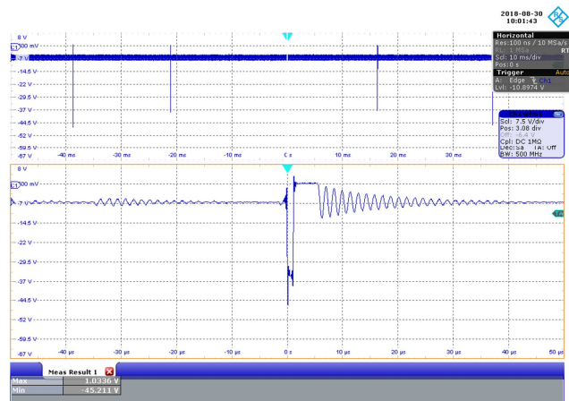
Figure 90 – 277 VAC 50 Hz, No-Load. CH1: 12 V FWL_DIODEF , 7.5 V / div., 10 ms / div. Zoom: 10 μs / div. 12 V PIV MAX = 45.211 V.
