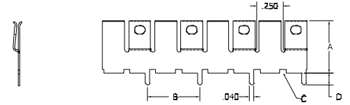
FIGURE 2 .50" Pin Spacing
