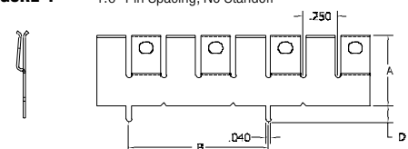
FIGURE 5 1.0" Pin Spacing, With Standoff
