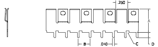
FIGURE 3 .25" Pin Spacing
