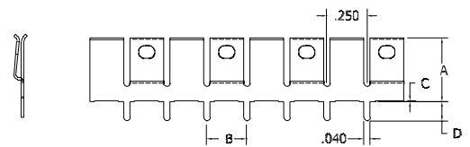
FIGURE 6 .25" Pin Spacing, With Standoff
