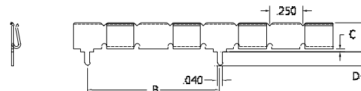
FIGURE 6 1.0" Pin Spacing, With Standoff
