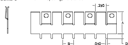
FIGURE 6 .25" Pin Spacing, No Standoff
