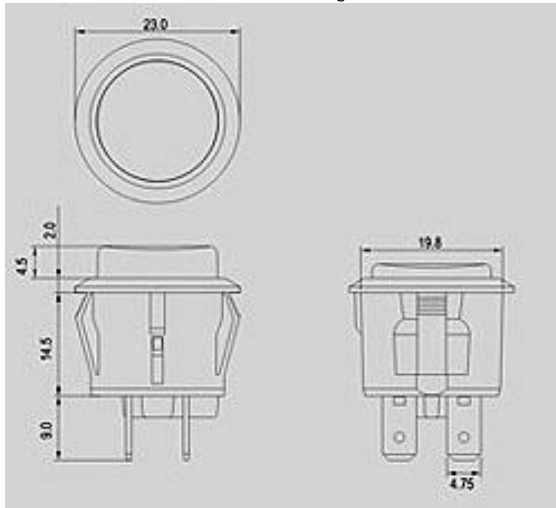
Outline Drawing
