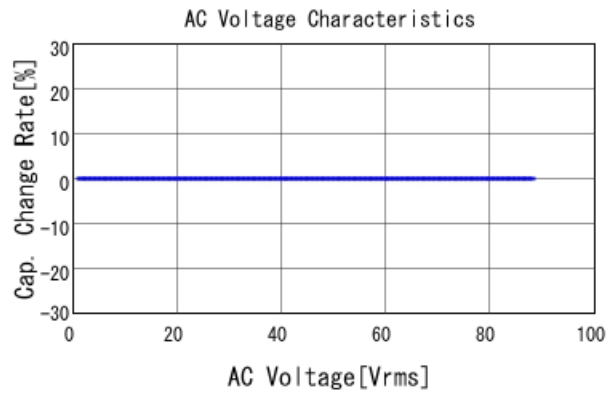
GRM21A5C2E470JW01 C-AC Voltage capchange, DCOV, 25
