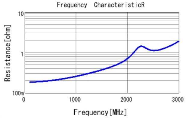
GRM21A5C2E470JW01 R DCOV, 25degC
