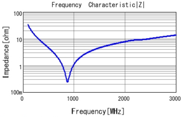
GRM21A5C2E470JW01 |Z| DCOV, 25degC
