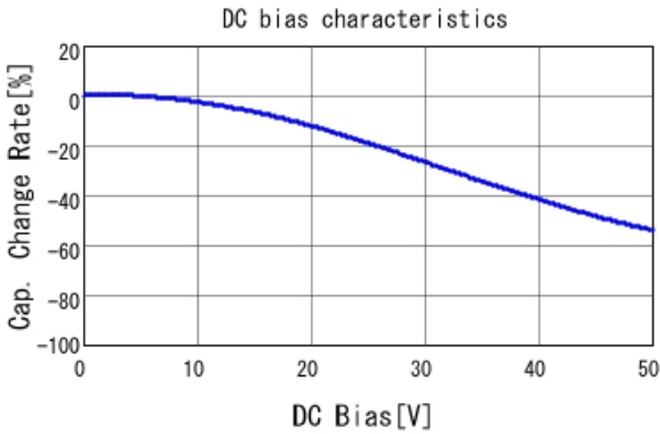
GRM033R71H221KA12 C-DC bias capchange, 25.0degC, A
