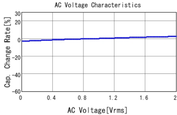
GRM033R71H221KA12 C-AC Voltage capchange, DCOV, 25
