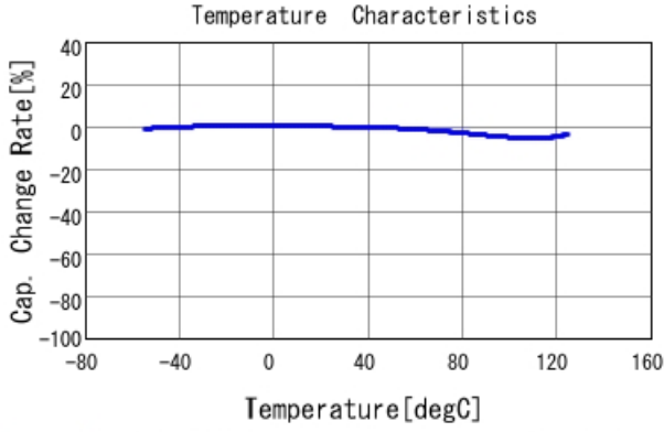
GRM033R71H221KA12 C-Temp. capchange, DC0.0V, AC1.C
