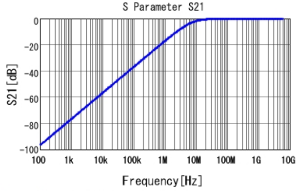
GRM033R71H221KA12 S21 DC0V, 25degC
