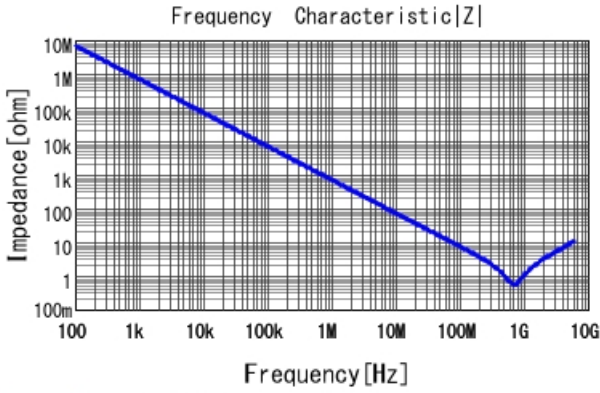
GRM033R71H221KA12 |Z| DCOV, 25degC
