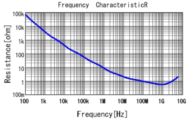
GRM033R71H221KA12 R DCOV, 25degC
