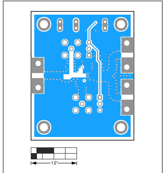
MAX40660 EV Kit PCB Layout—Bottom Layer
