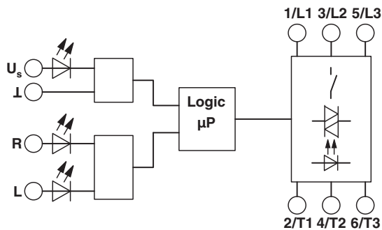
Figure 3 Block diagram
