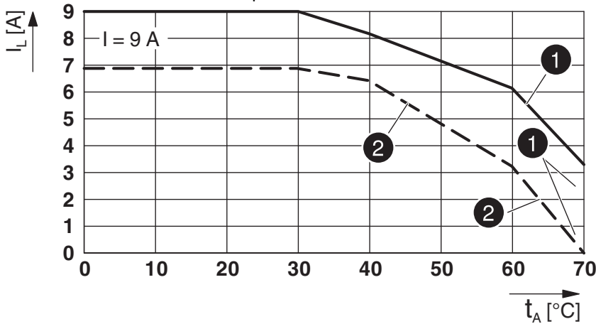
Figure 4 Derating curve
