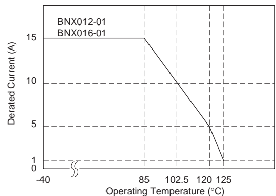
Derating
