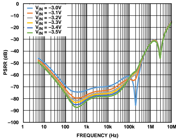
Figure 32. Power Supply Rejection Ratio (PSRR) vs. Frequency at Various Input Voltages, V_{OUT} = -2.5 V , I_{LOAD} = -300 mA
