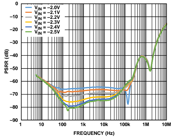
Figure 31. Power Supply Rejection Ratio (PSRR) vs. Frequency at Various Input Voltages, V_{OUT} = -1.2 V , I_{LOAD} = -300 mA
