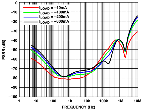
Figure 29. Power Supply Rejection Ratio (PSRR) vs. Frequency at Various Loads, V_{OUT} = -2.5 V , V_{IN} = -3 V
