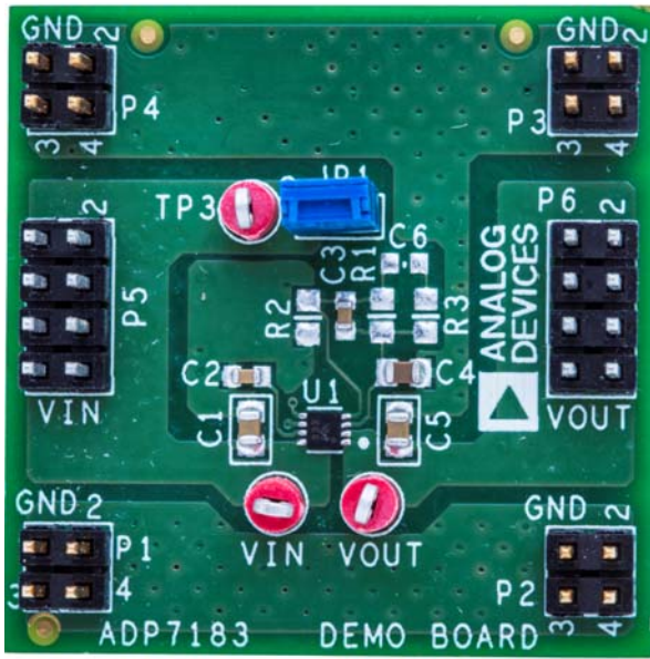
Figure 53. Evaluation Board
