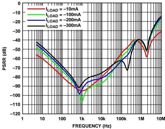
Figure 30. Power Supply Rejection Ratio (PSRR) vs. Frequency at Various Loads, V_{OUT} = -3.3 V , V_{IN} = -3.8 V
