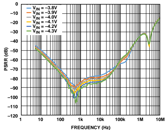
Figure 33. Power Supply Rejection Ratio (PSRR) vs. Frequency at Various Input Voltages, V_{OUT} = -3.3 V , I_{LOAD} = -300 mA
