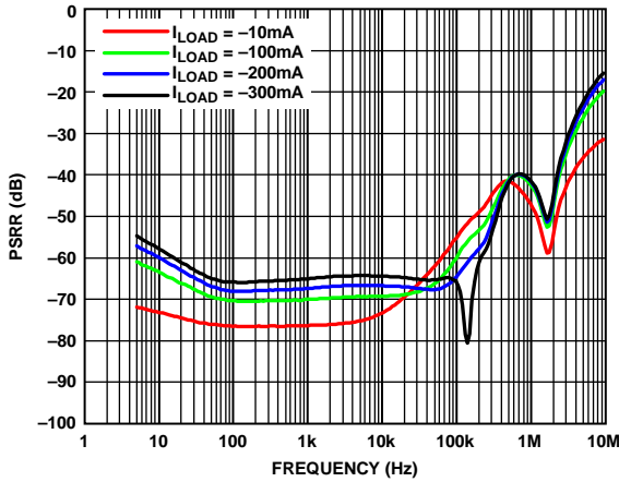
Figure 28. Power Supply Rejection Ratio (PSRR) vs. Frequency at Various Loads, V_{OUT} = -1.2 V , V_{IN} = -2 V
