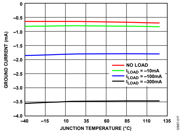
Figure 7. Ground Current vs. Junction Temperature ( T_J ), V_{OUT} = -1.2\text{ V}
