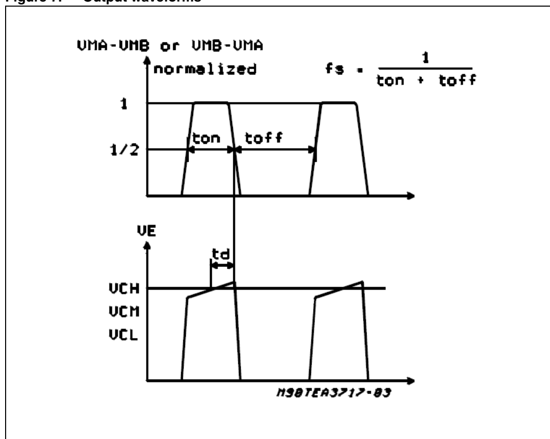
Figure 7. Output waveforms
