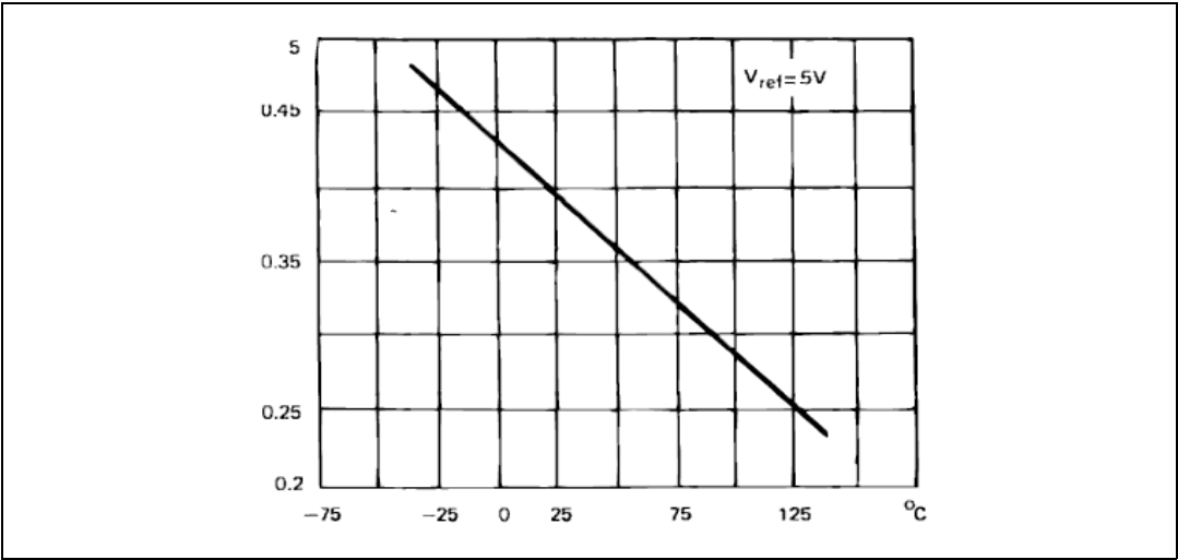
Figure 12. I_{ref} against junction temperature
