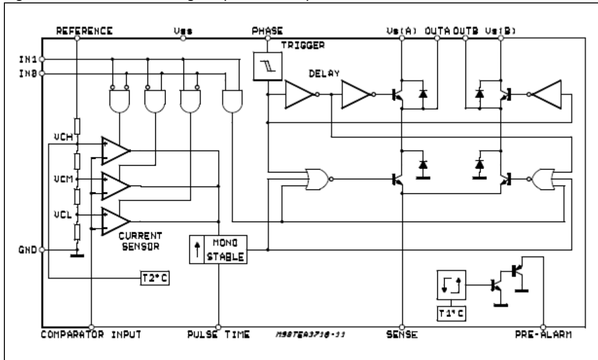
Figure 3. Detailed block diagram (TEA3718SFP)
