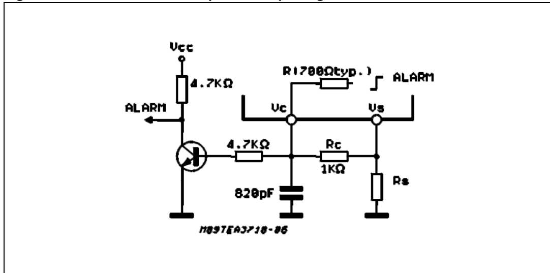
Figure 16. Alarm detection for power DIP package
