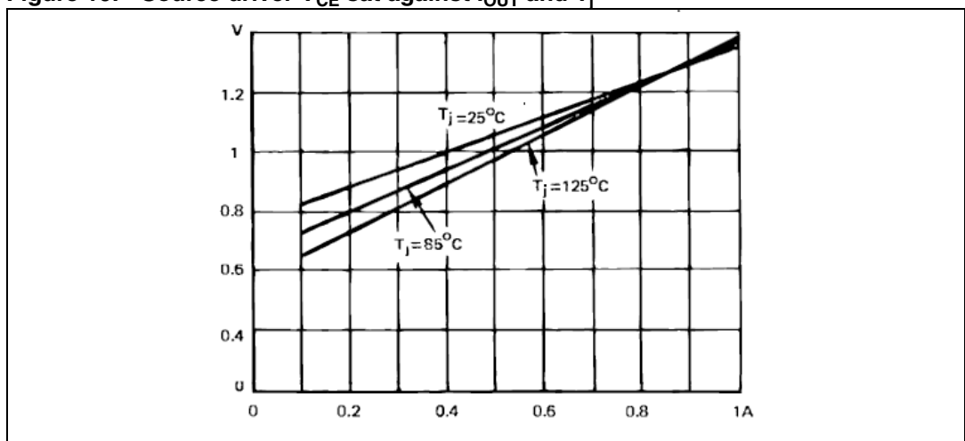
Figure 10. Source driver V_{CE\text{ sat}} against I_{OUT} and T_j
