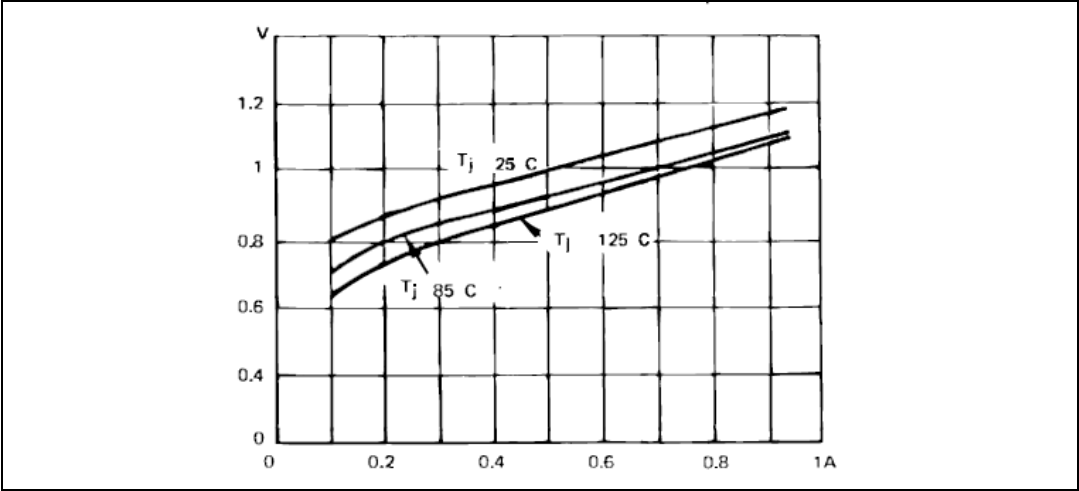
Figure 11. Upper diode V_f against I_{OUT} and T_j
