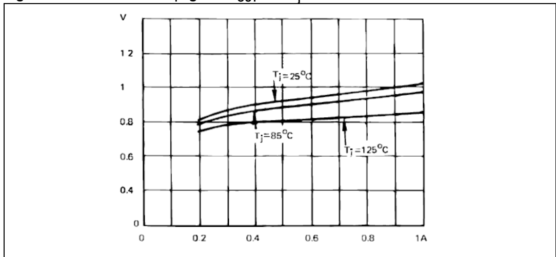
Figure 10. Source driver V_{CE\text{ sat}} against I_{OUT} and T_j
