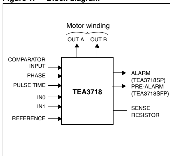
Figure 1. Block diagram
