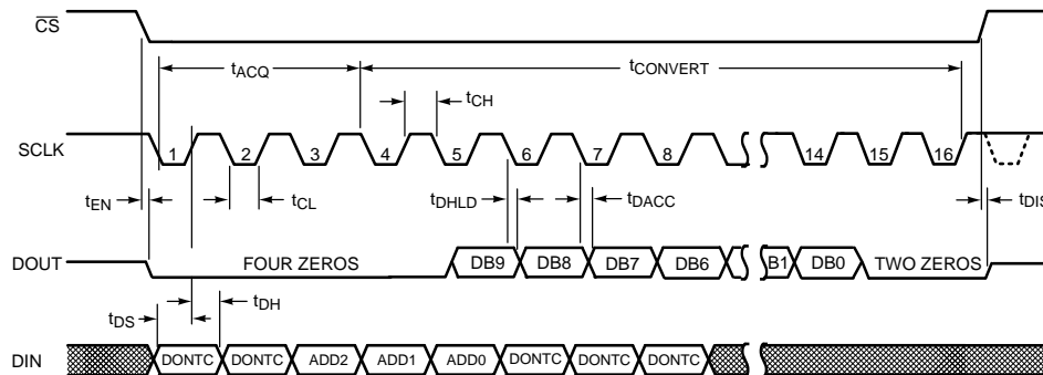
Figure 3. ADC108S022 Serial Timing Diagram
